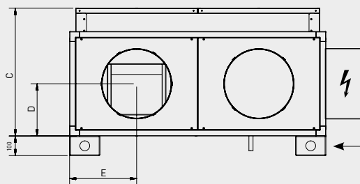
Support feet (models 45, 55 and 80). Only location on flat surface.
