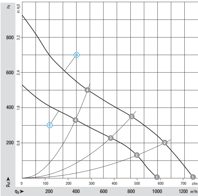
Curves (Speed-controlled)
